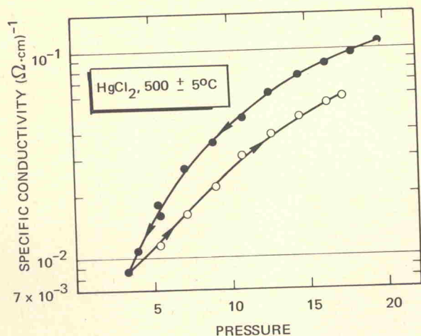
FIG. 4. Isothermal specific conductance ( K ) of \text{HgCl}_2 as a function of pressure (kbar).
