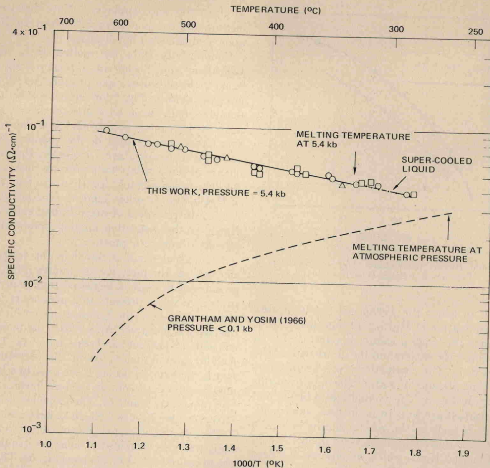
Fig. 5. \text{Log}K(\Omega\cdot\text{cm})^{-1} vs 1/T ( ^{\circ}\text{K} ) for \text{HgI}_2 . (O) Sample No. 3, Run No. 3; (□) Sample No. 3, Run No. 4; (△) Sample No. 4, Run No. 1. Pressures given in kbars.
